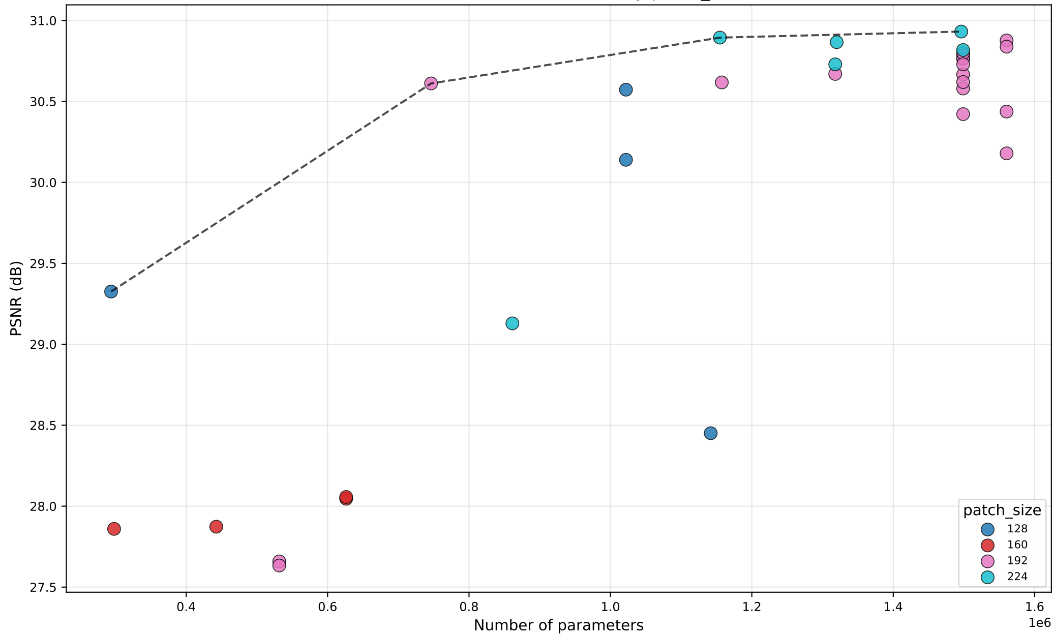
PSNR vs #Params — DAT — by patch_size
